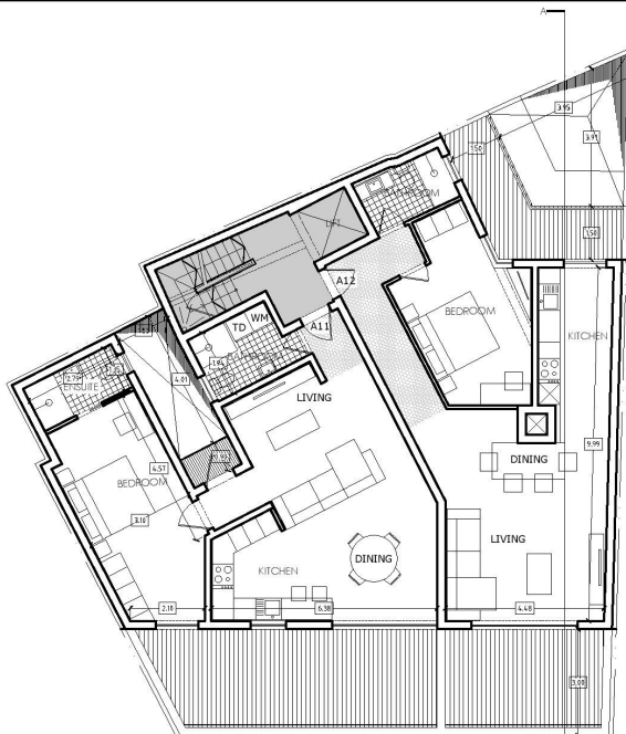
PROPOSED LEVEL 6 SCALE 1:100
