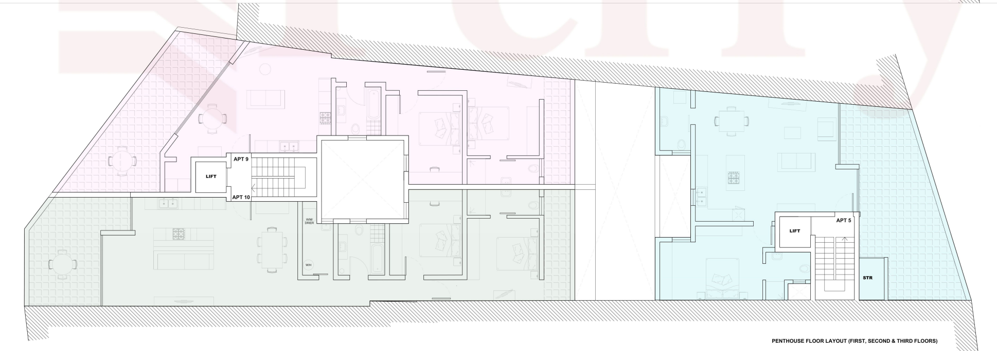
TYPICAL FLOOR LAYOUT (FIRST, SECOND & THIRD FLOORS)
