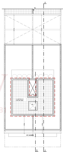
Proposed Over Roof Plan Scale 1/100
