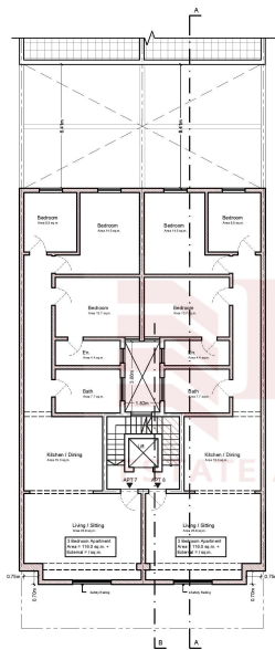
Proposed Third Floor Plan Scale 1/100
