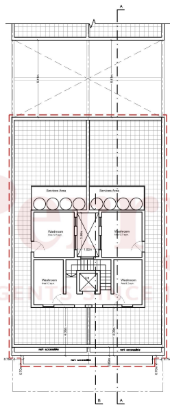
Proposed Fourth (Roof) Floor Plan Scale 1/100
