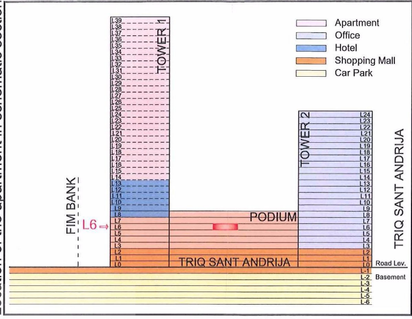
Location of the apartment in schematic section
