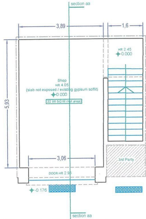
GROUND FLOOR LEVEL scale 1:100
