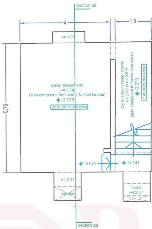
BASEMENT LEVEL scale 1:100
