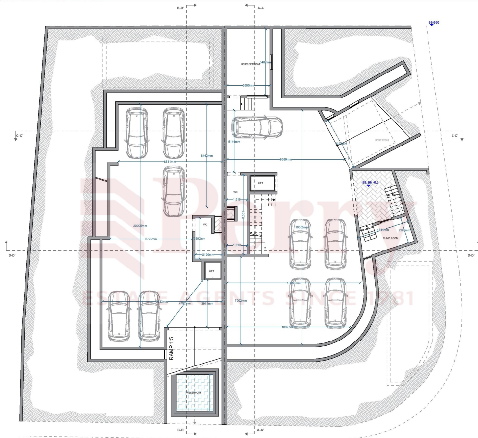
PROPOSED BASEMENT LEVEL -1 scale 1:100
