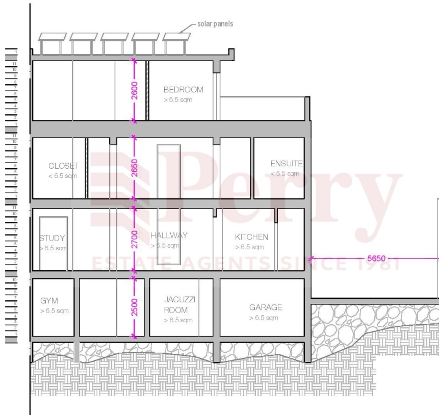
existing section bb
