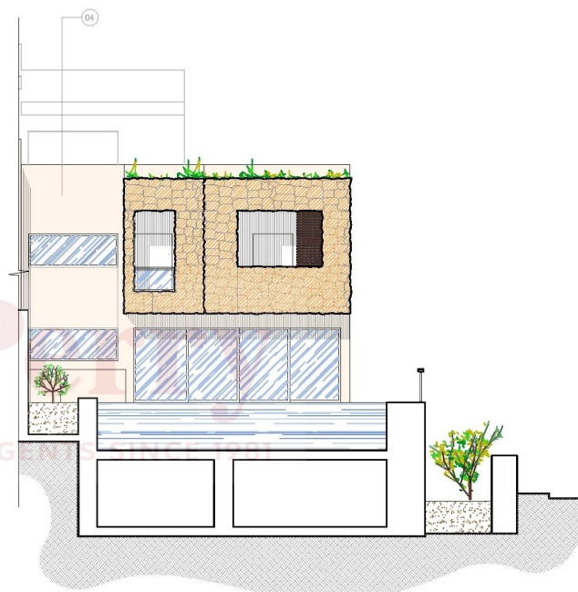
Proposed Elevation 'A3' Scale 1:100
