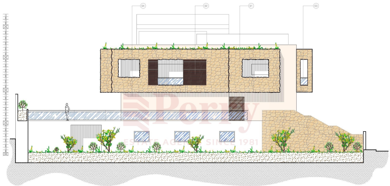
Proposed Elevation 'A4' Scale 1:100
