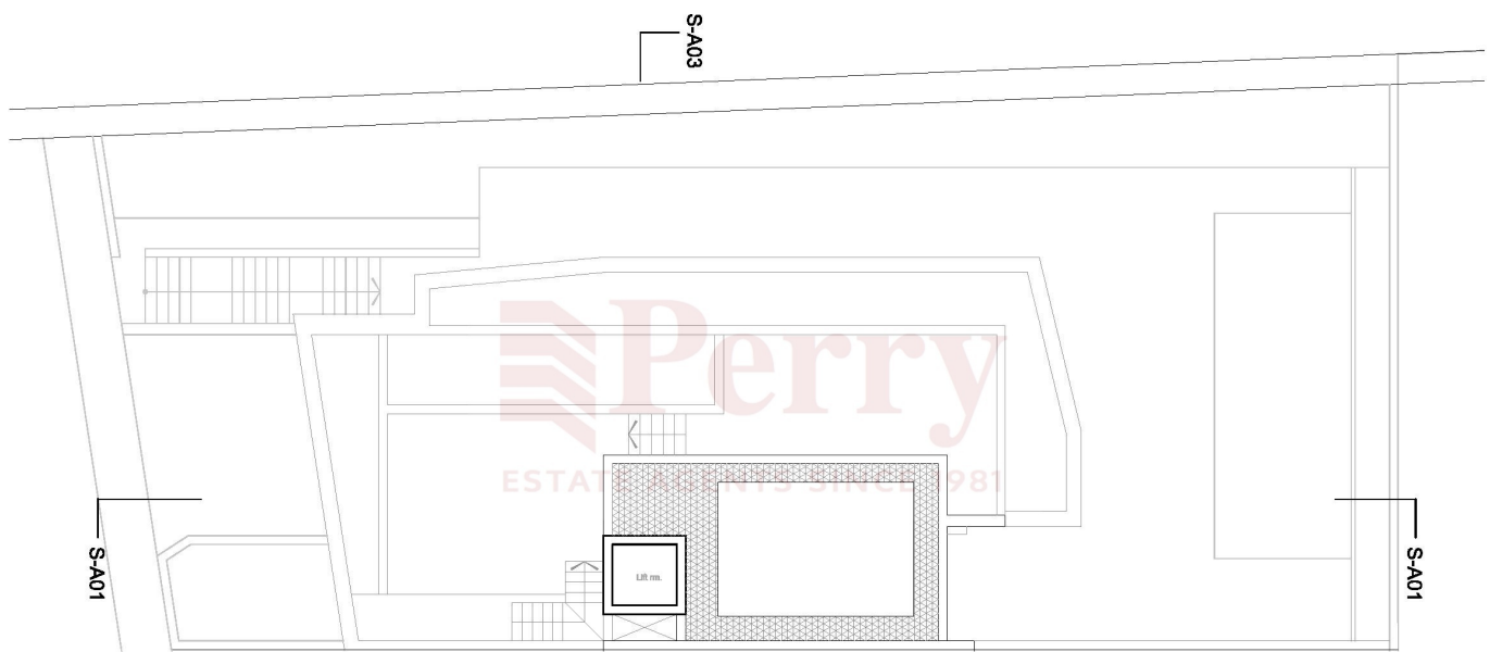
Proposed Roof over Second Floor Level Scale 1:100
