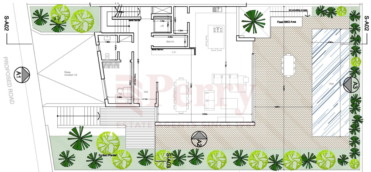
Proposed Ground Floor Level Scale 1:100
