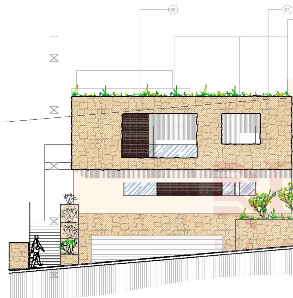
Proposed Elevation 'B1' Scale 1:100
