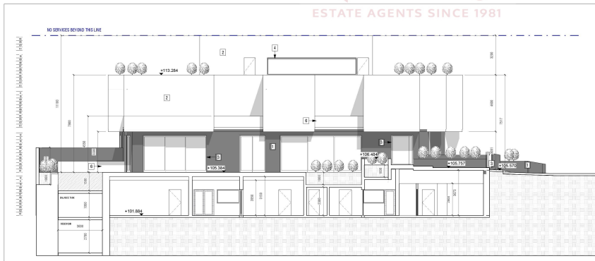
V1 SECTION 2 PROPOSED SCALE 1 : 100
