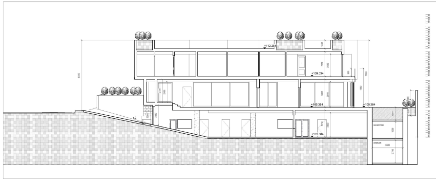
V1 SECTION 1 PROPOSED SCALE 1 : 100
